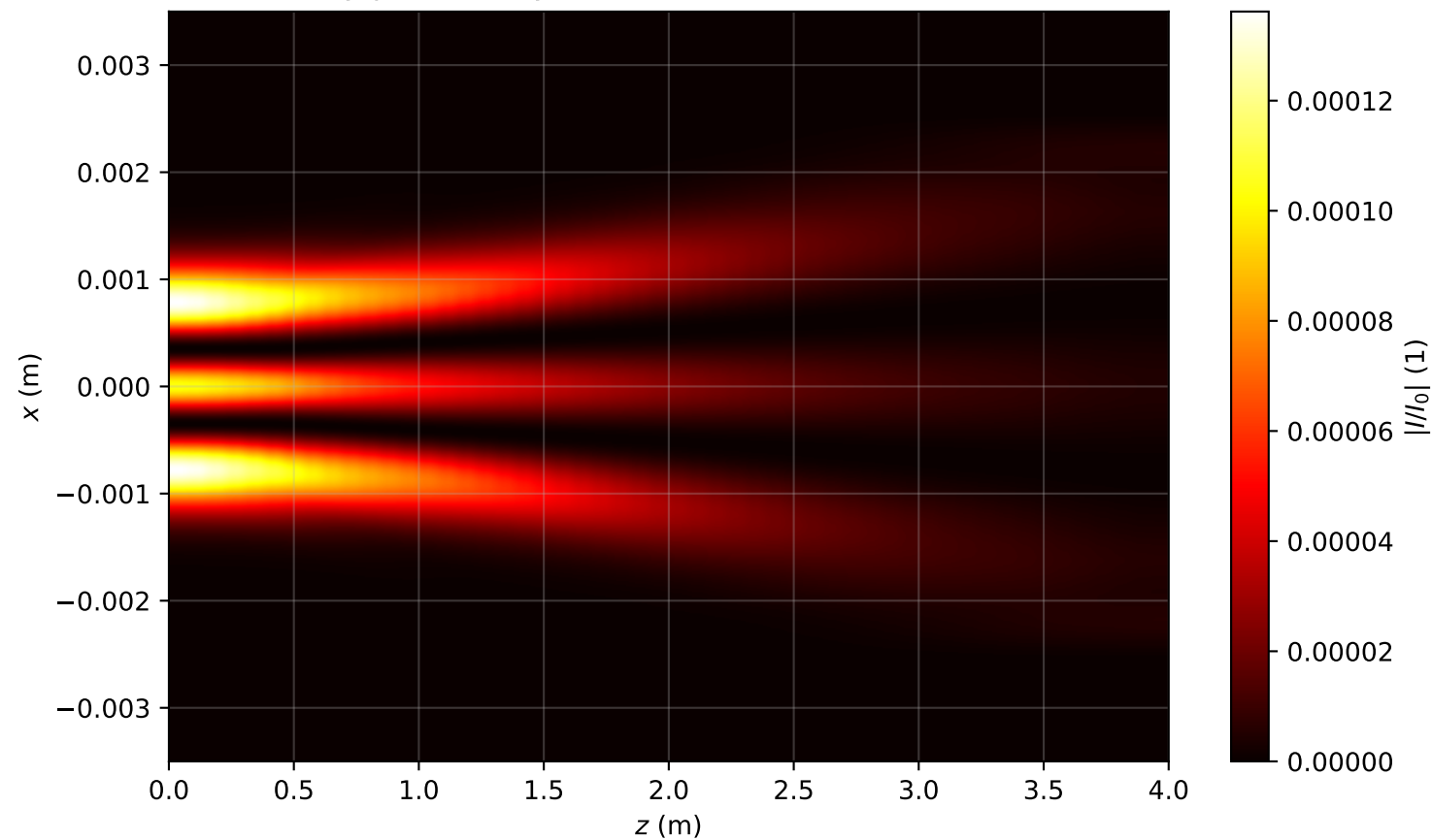
Intensity profile I(x, y = 0, z)/I_0 , P_{in}=1.0P_{cr} , artificial time
